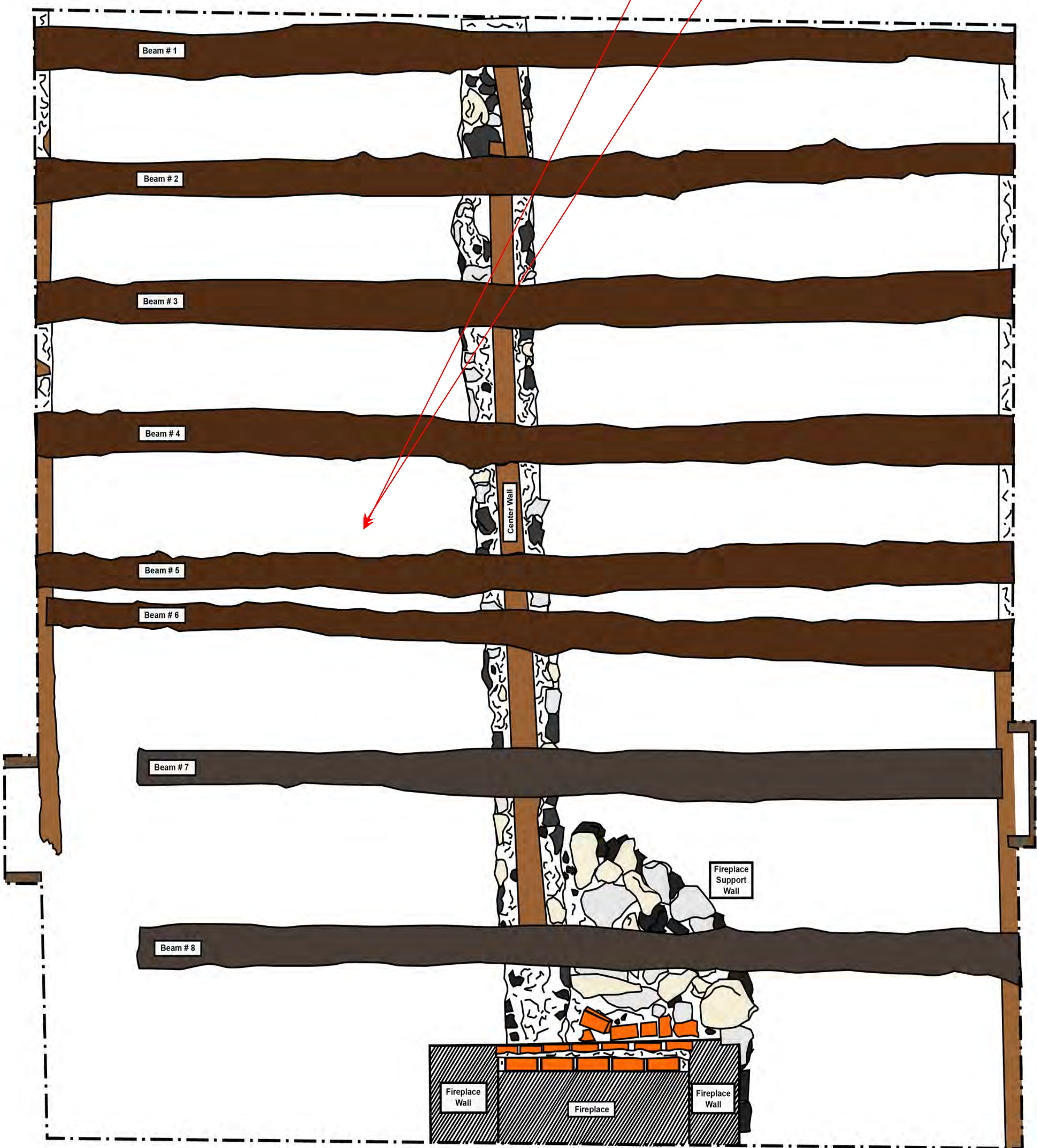
CATOCTIN, FORGEMAN HOUSE FLOOR PLAN
